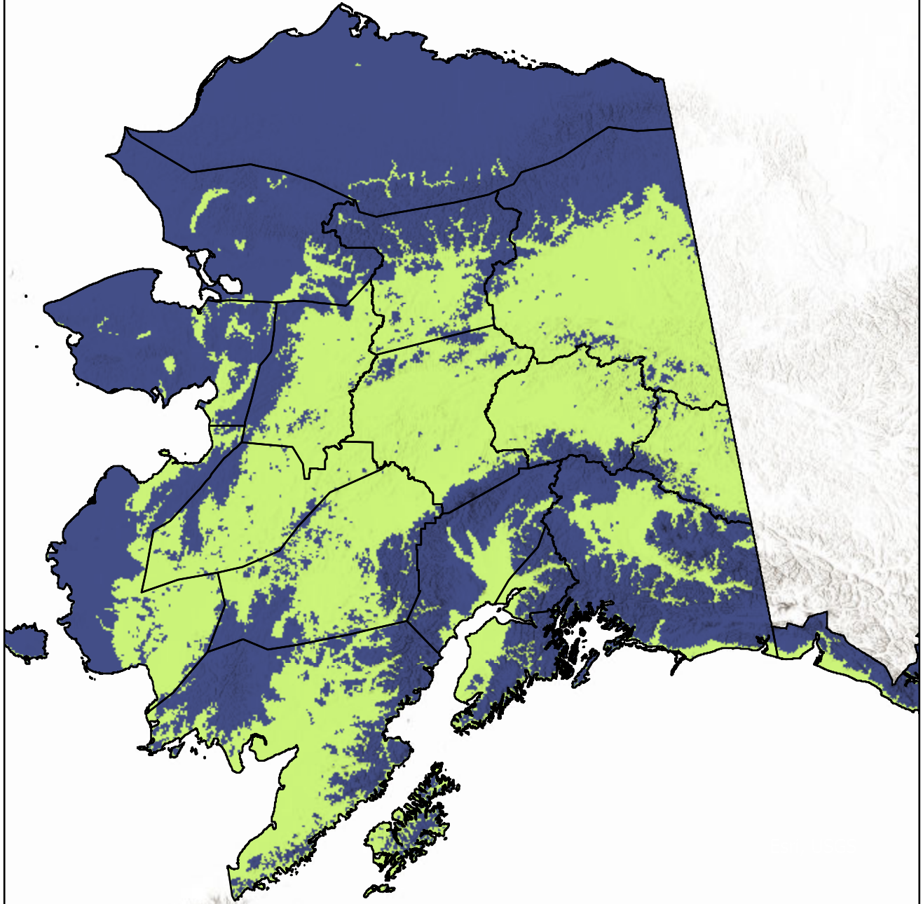
US National Ice Center IMS as Snow On/Off
